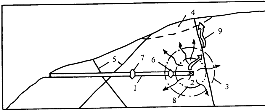
Figure 19. Illustration of gas release through a tectonic fault: 1- tunnel works; 2- zero room; 3- damage zone radius; 4- spill zone; 5- faults; 6 and 7- first and second stemming; 8- outer boundary of area in which the gas is moving through the damaged rock massif; 9- gas flow through the tectonic fault.
